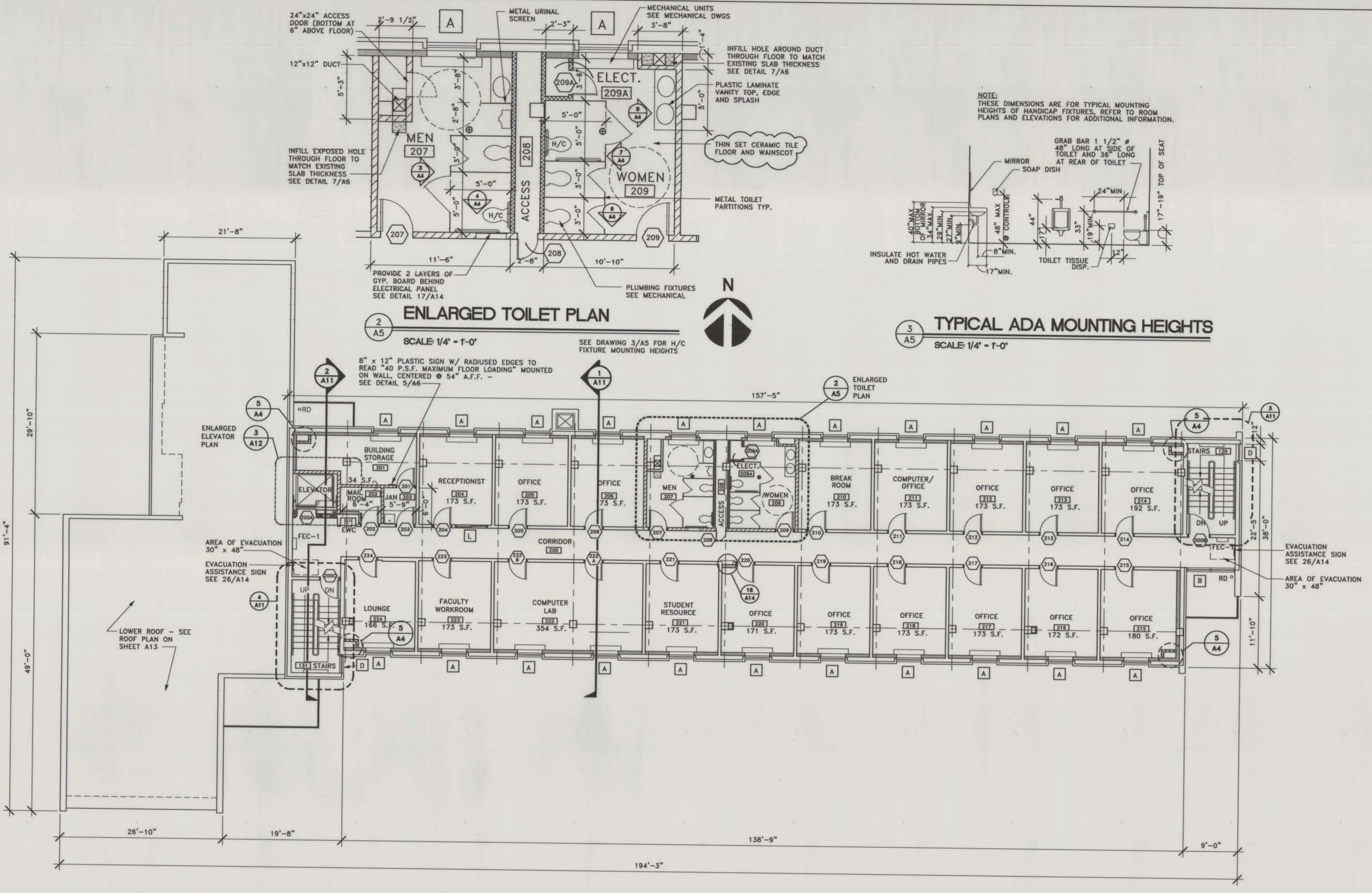
1 A5 RENOVATED PLAN - 2ND FLOOR SCALE: 1/8" = 1'-0"
