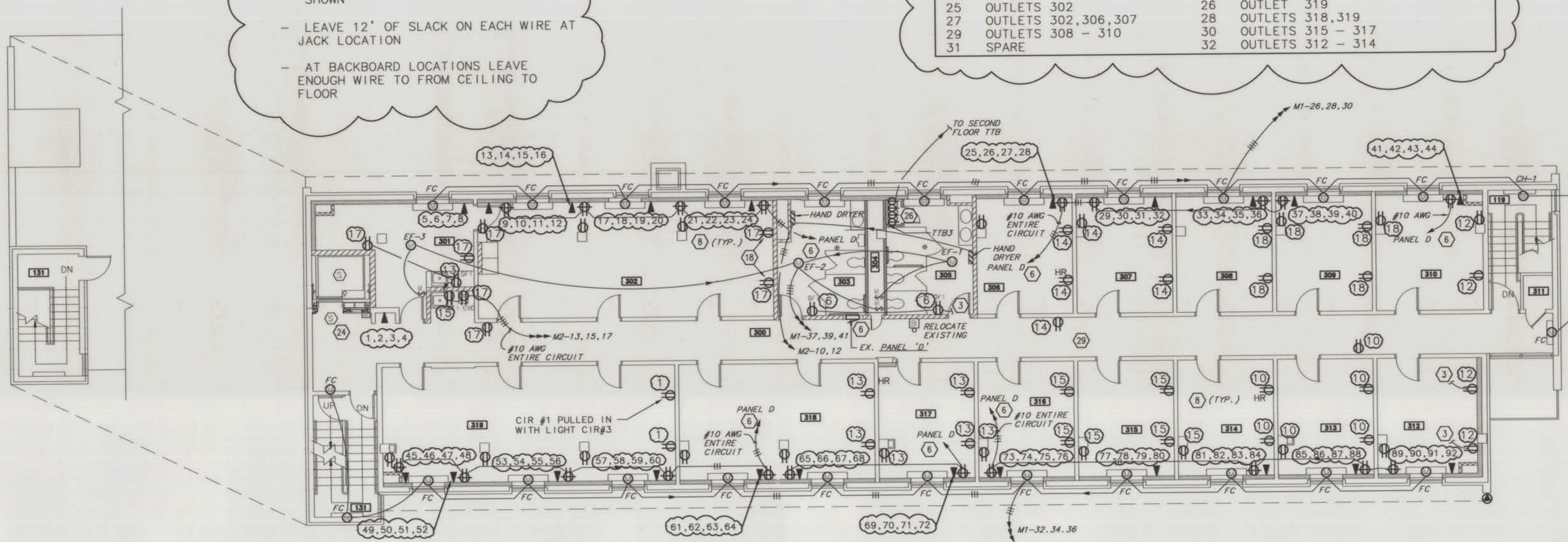
2 E6 THIRD FLOOR PLAN POWER 1/8"=1'-0"
